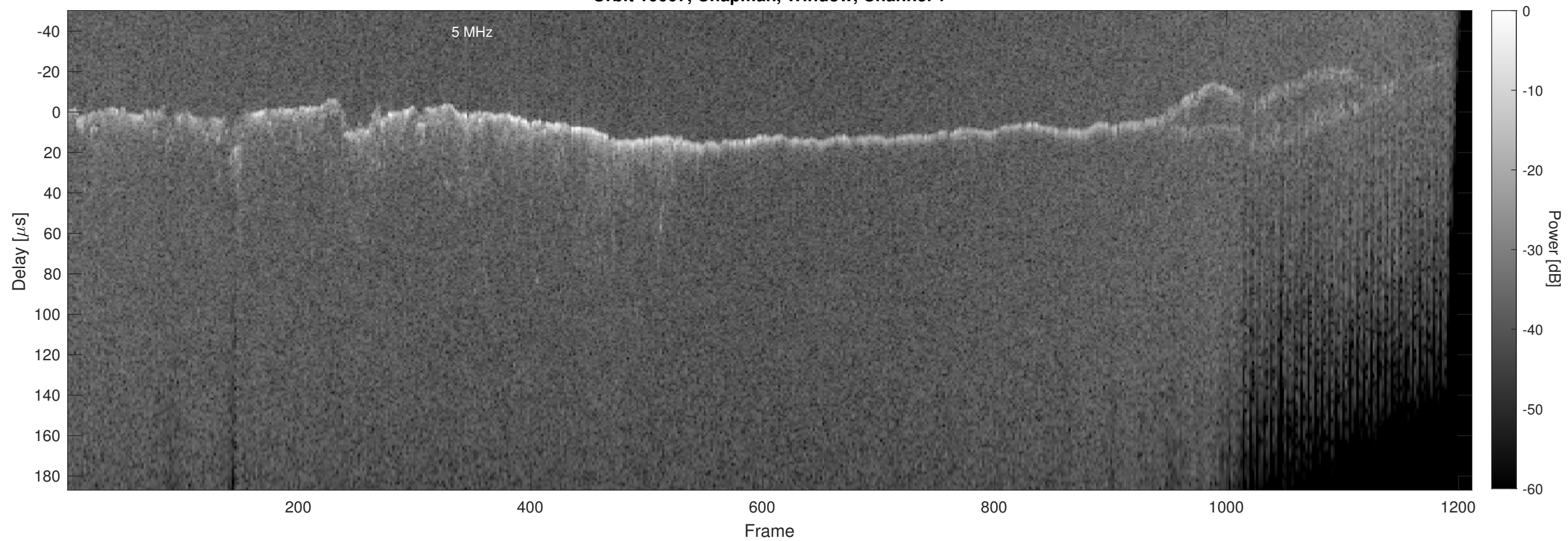
Orbit 10007, Chapman, Window, Channel 2
