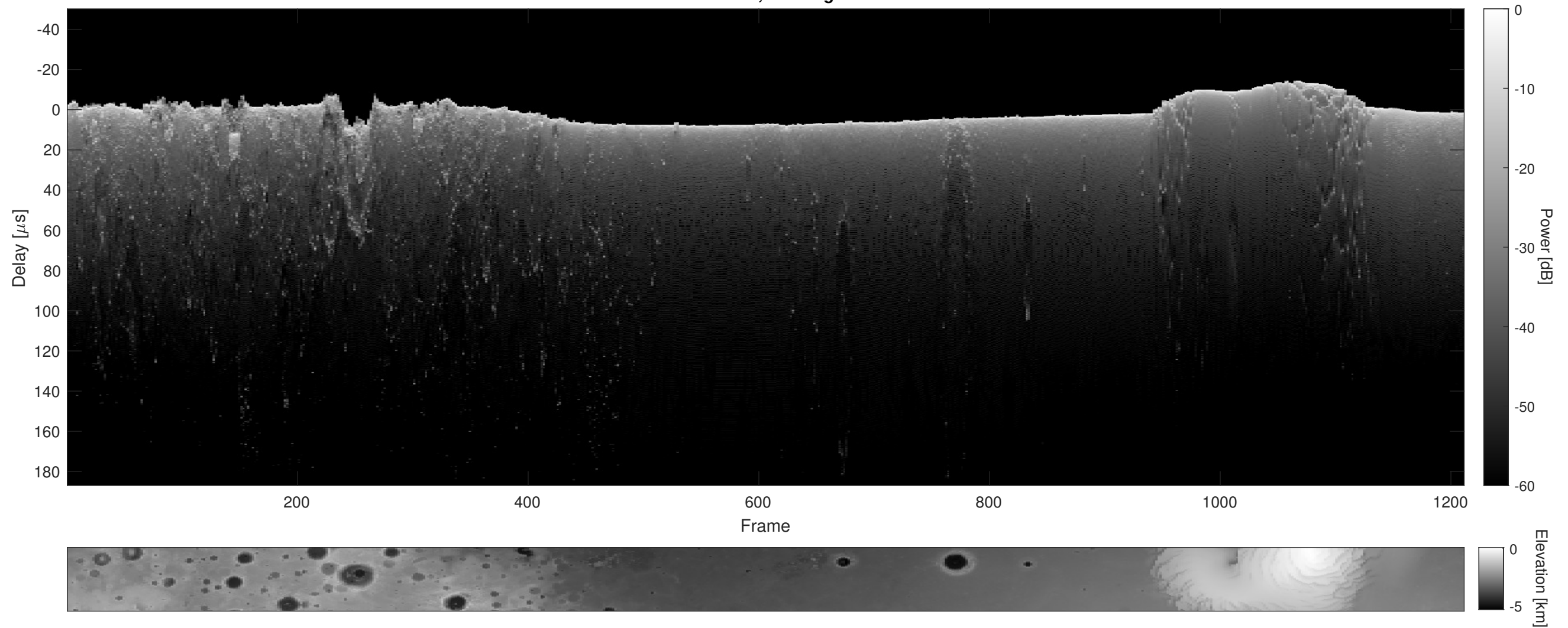
Orbit 10007, Cluttergram
