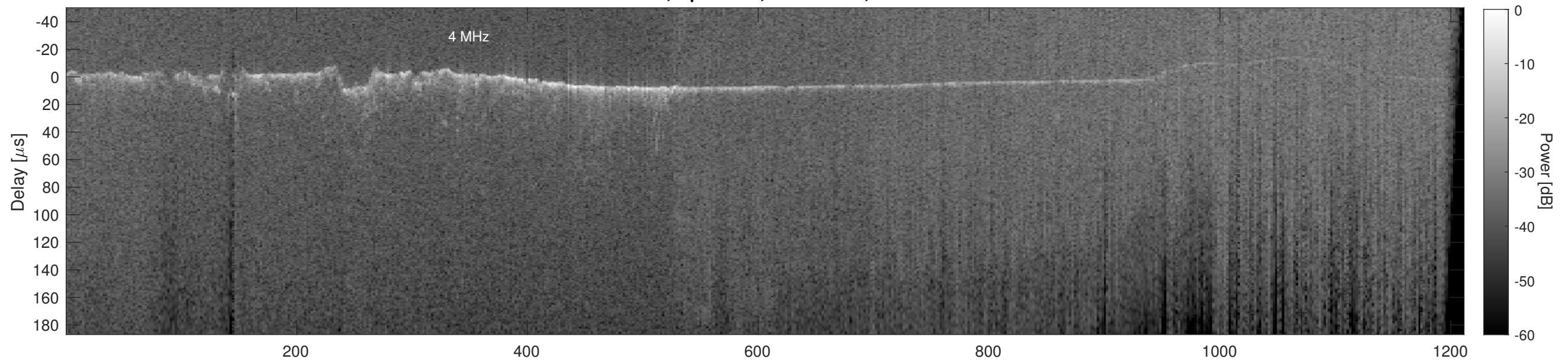
Orbit 10007, Cluttergram
