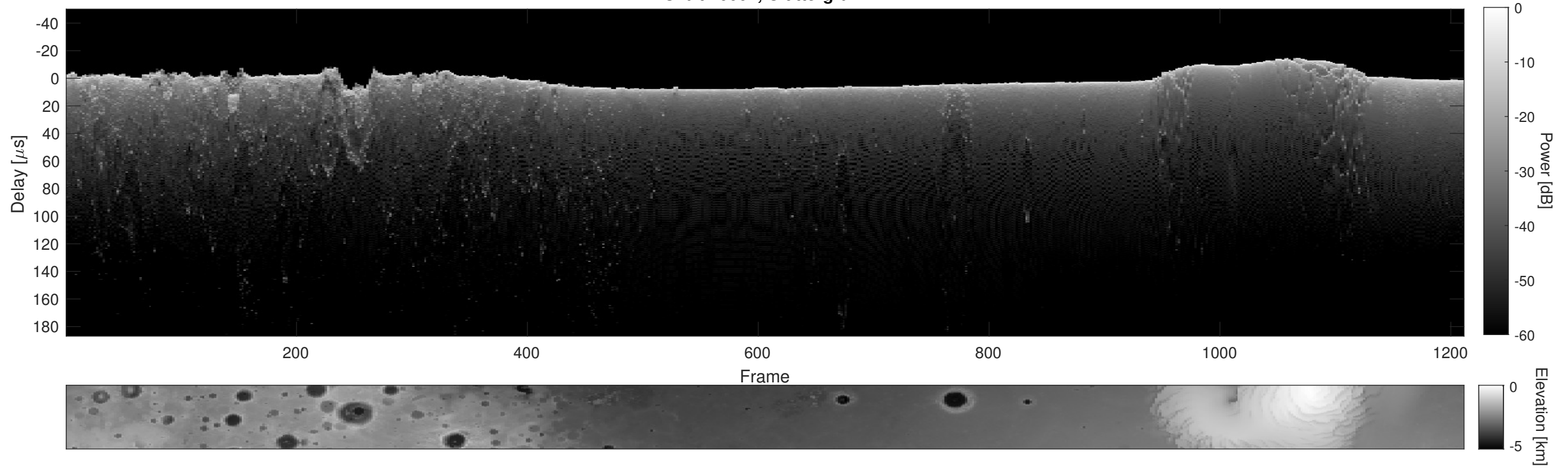
Orbit 10007, Cluttergram
