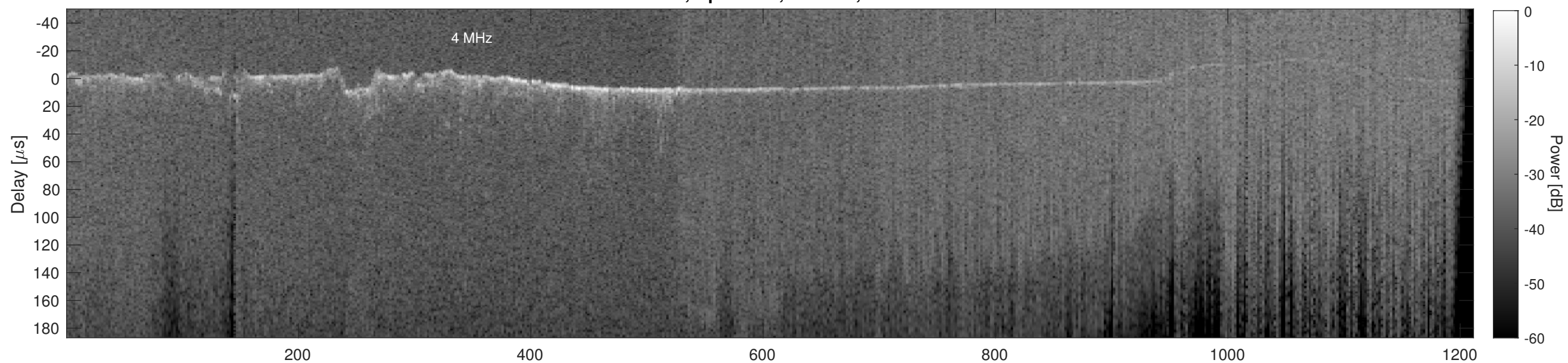
Orbit 10007, Cluttergram
