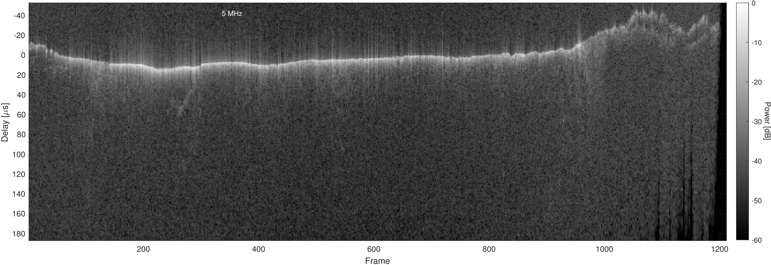
Orbit 10012, Chapman, No Window, Channel 2
