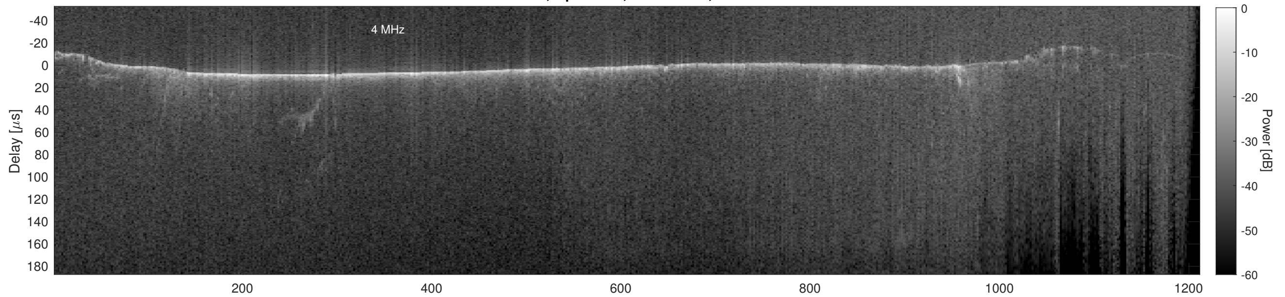
Orbit 10012, Cluttergram
