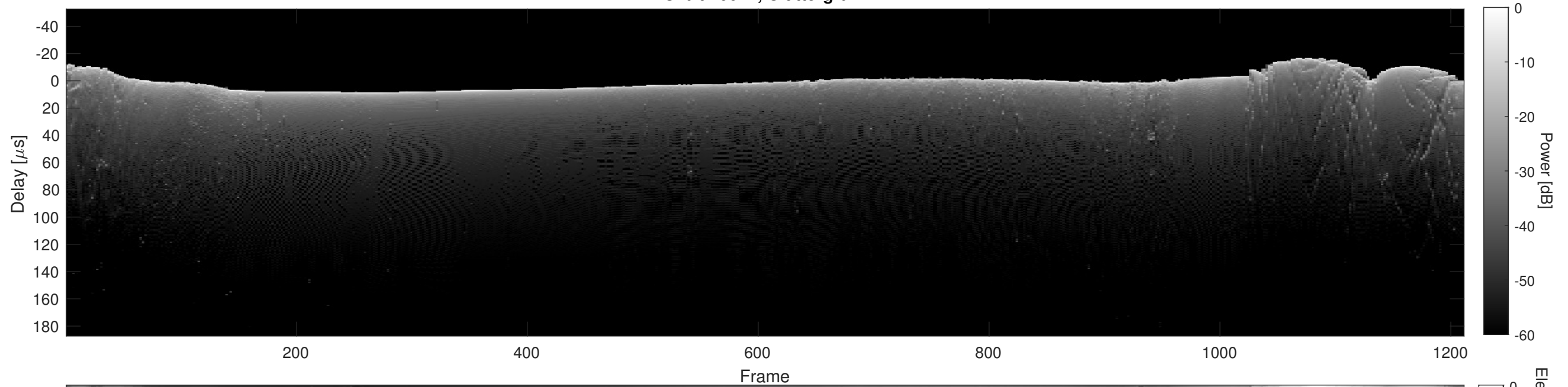
Orbit 10012, Cluttergram
