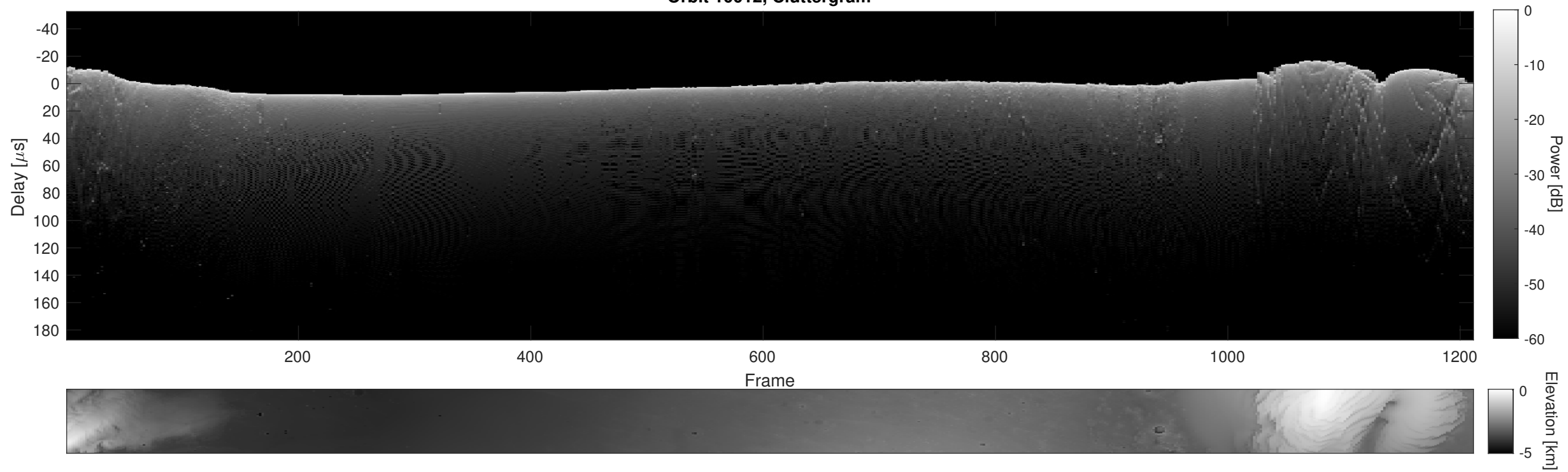
Orbit 10012, Cluttergram
