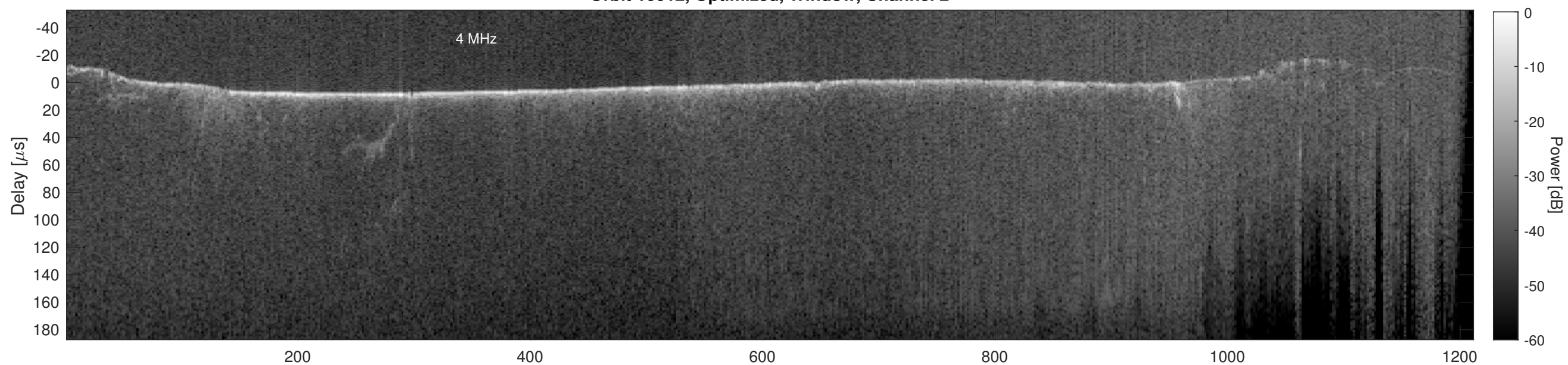
Orbit 10012, Cluttergram
