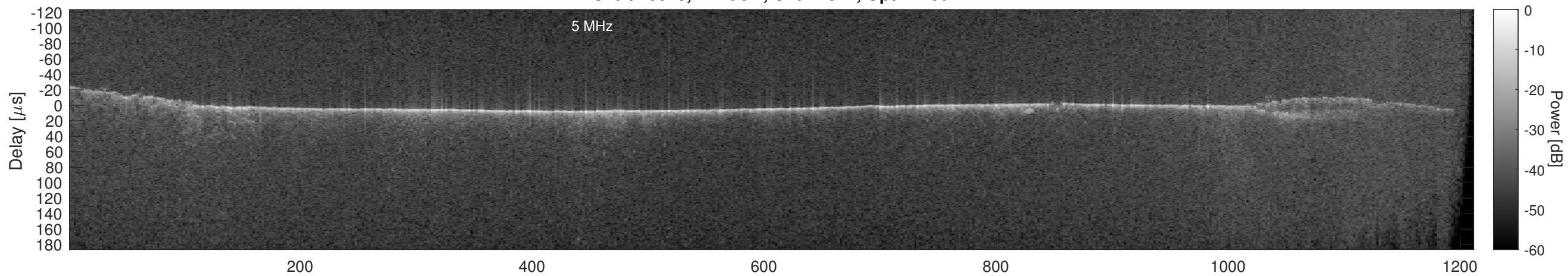
Orbit 10013, Cluttergram
