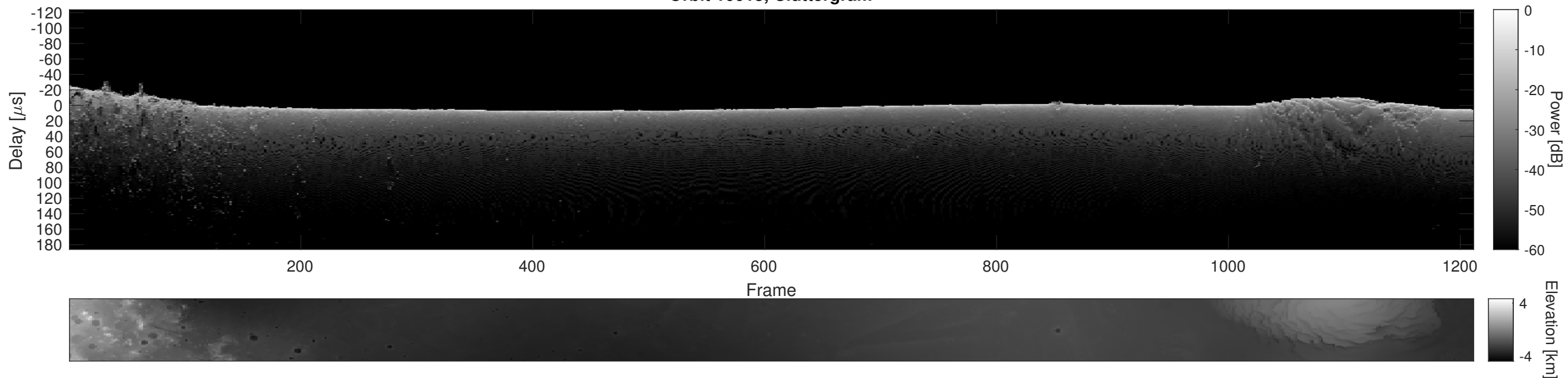
Orbit 10013, Cluttergram
