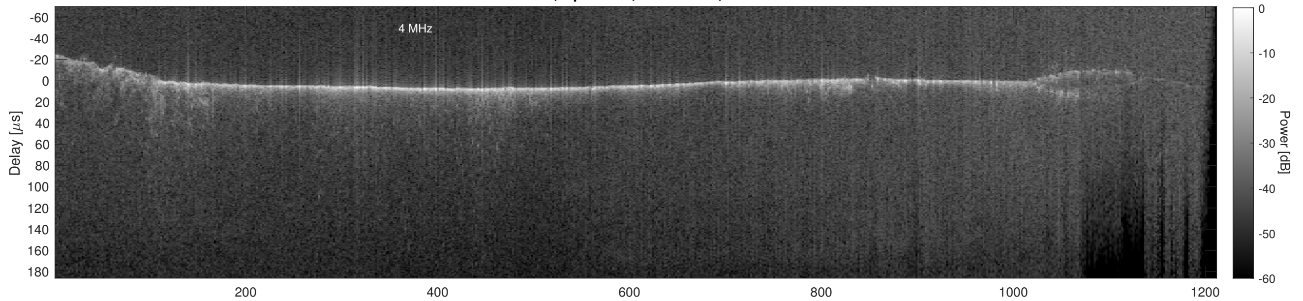
Orbit 10013, Cluttergram
