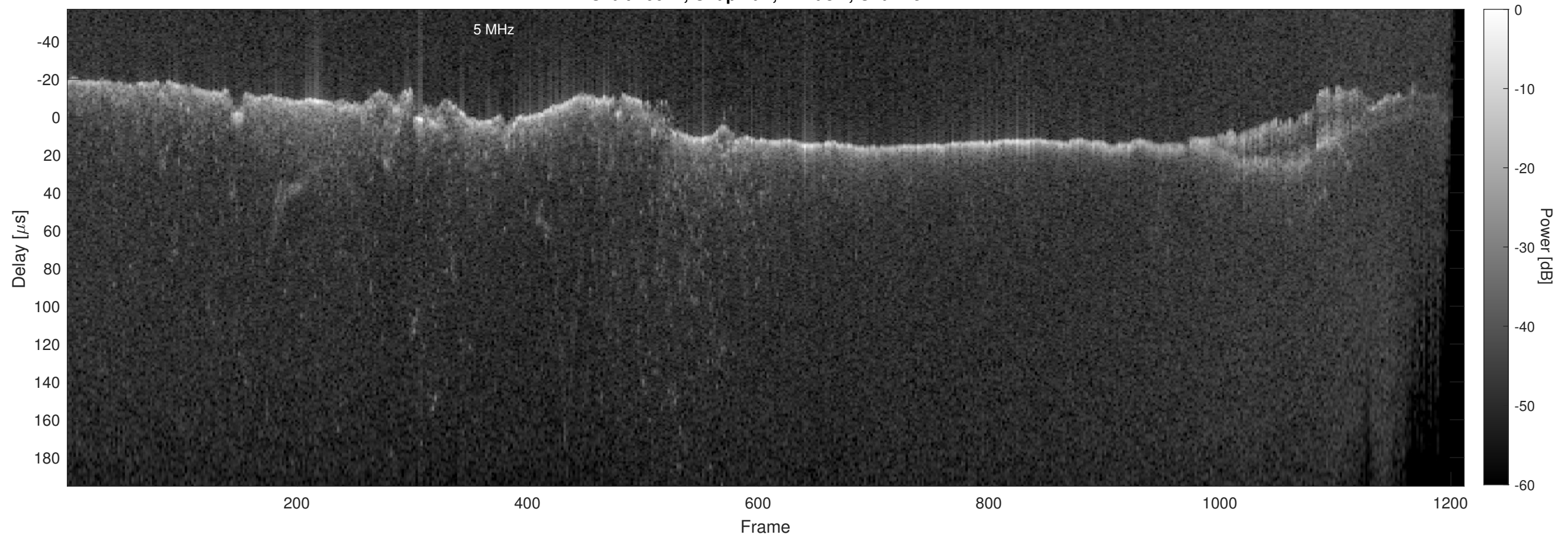
Orbit 10017, Chapman, Window, Channel 2
