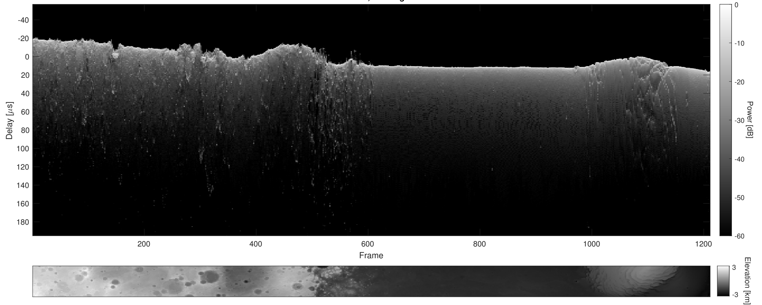
Orbit 10017, Cluttergram
