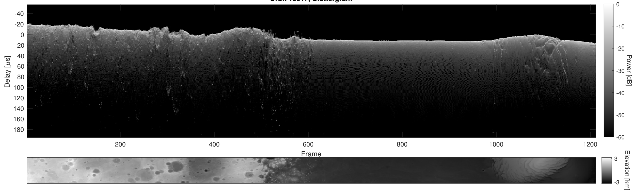
Orbit 10017, Cluttergram
