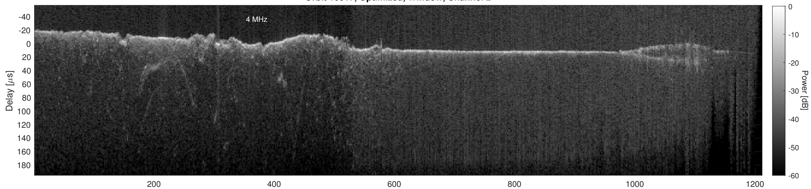
Orbit 10017, Cluttergram
