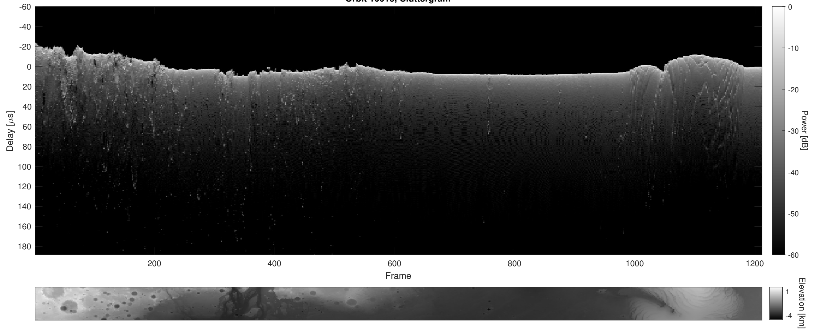
Orbit 10018, Cluttergram
