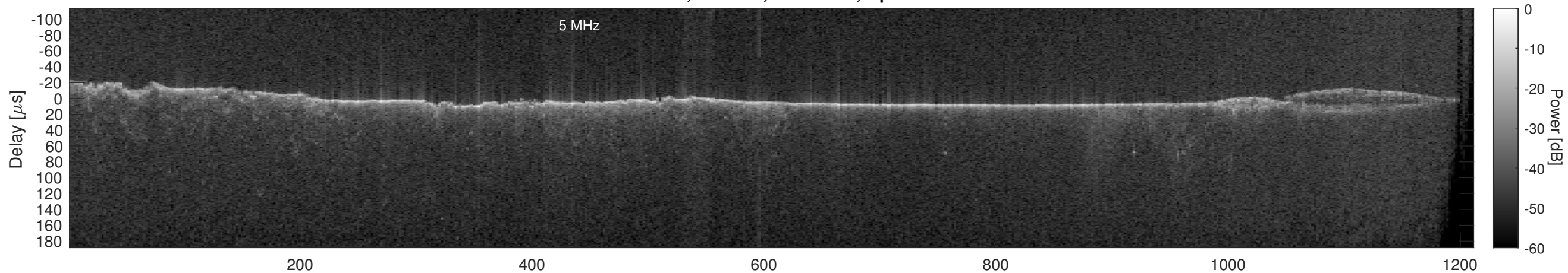
Orbit 10018, Cluttergram
