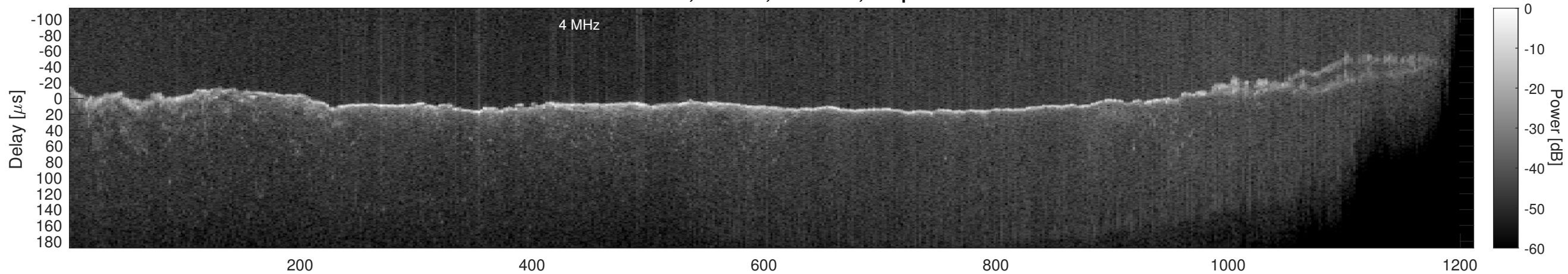
Orbit 10018, Window, Channel 2, Optimized
