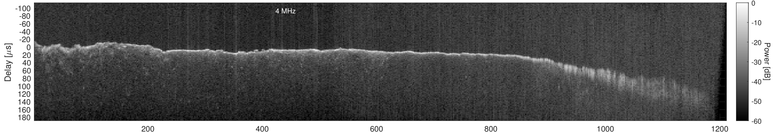
Orbit 10018, Window, Channel 2, Chapman
