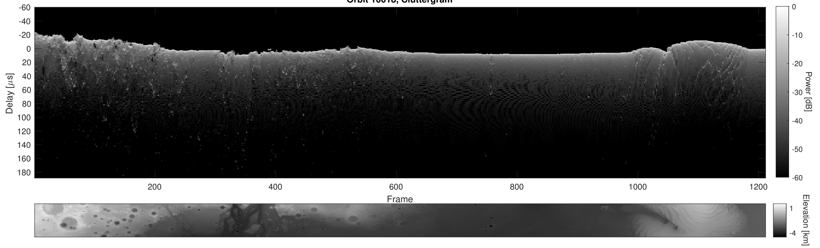
Orbit 10018, Cluttergram
