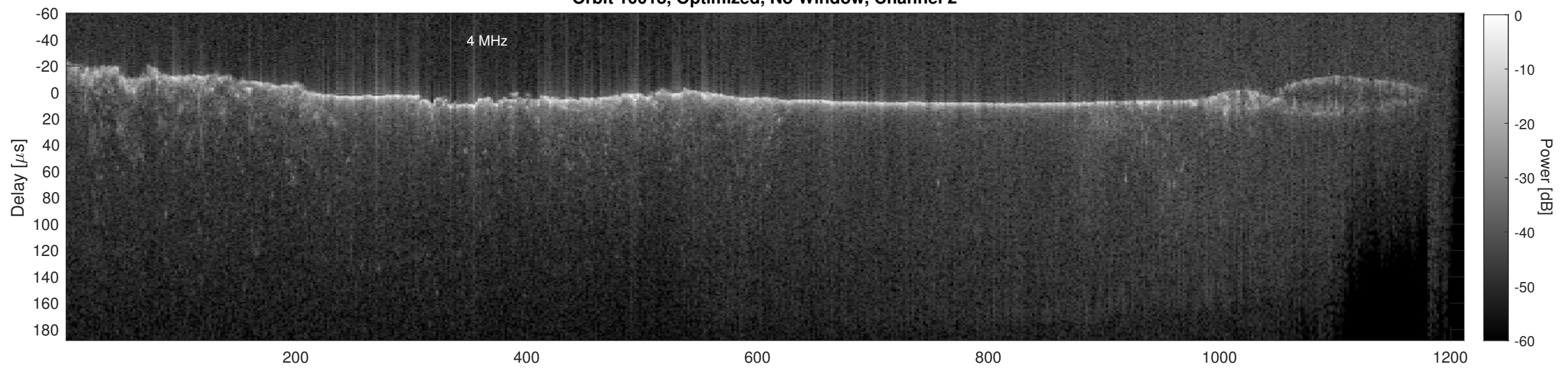
Orbit 10018, Cluttergram
