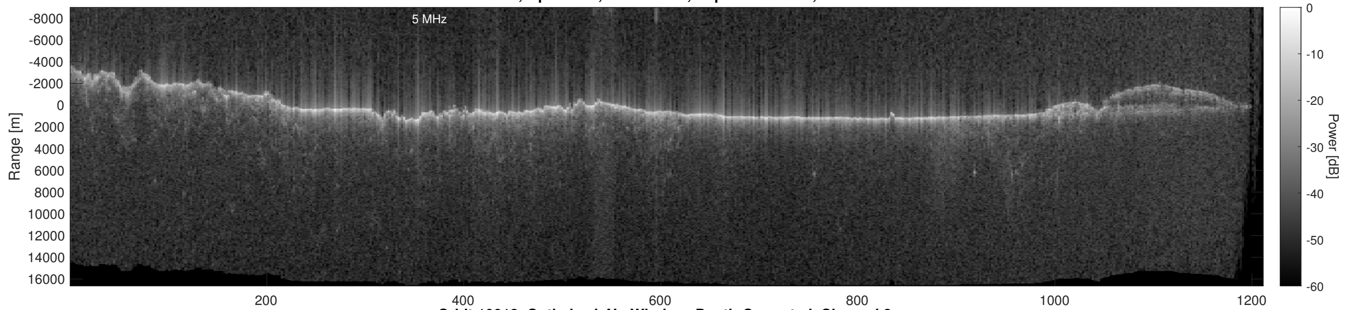
Orbit 10018, Optimized, No Window, Depth-Corrected, Channel 2
