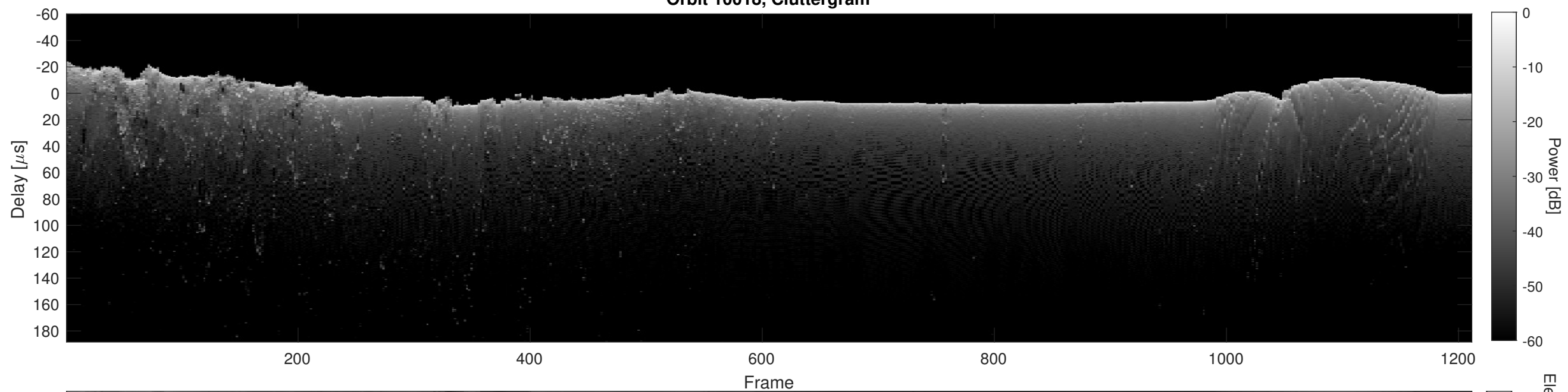
Orbit 10018, Cluttergram
