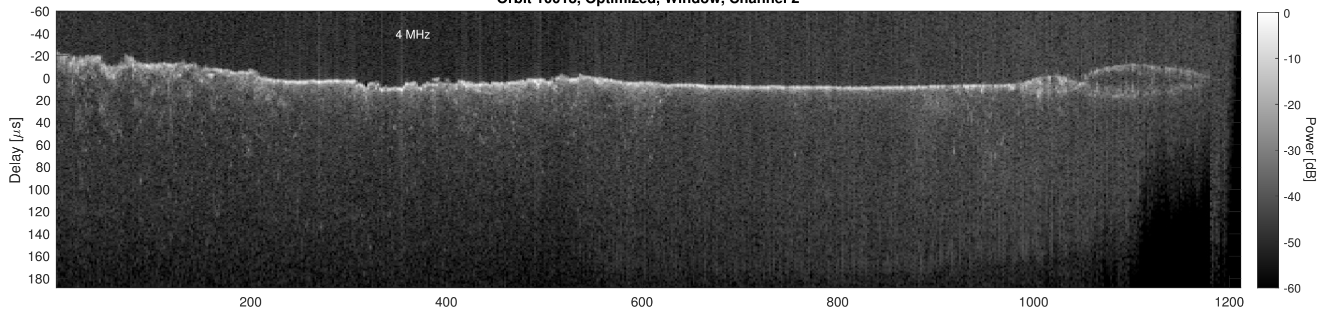
Orbit 10018, Cluttergram
