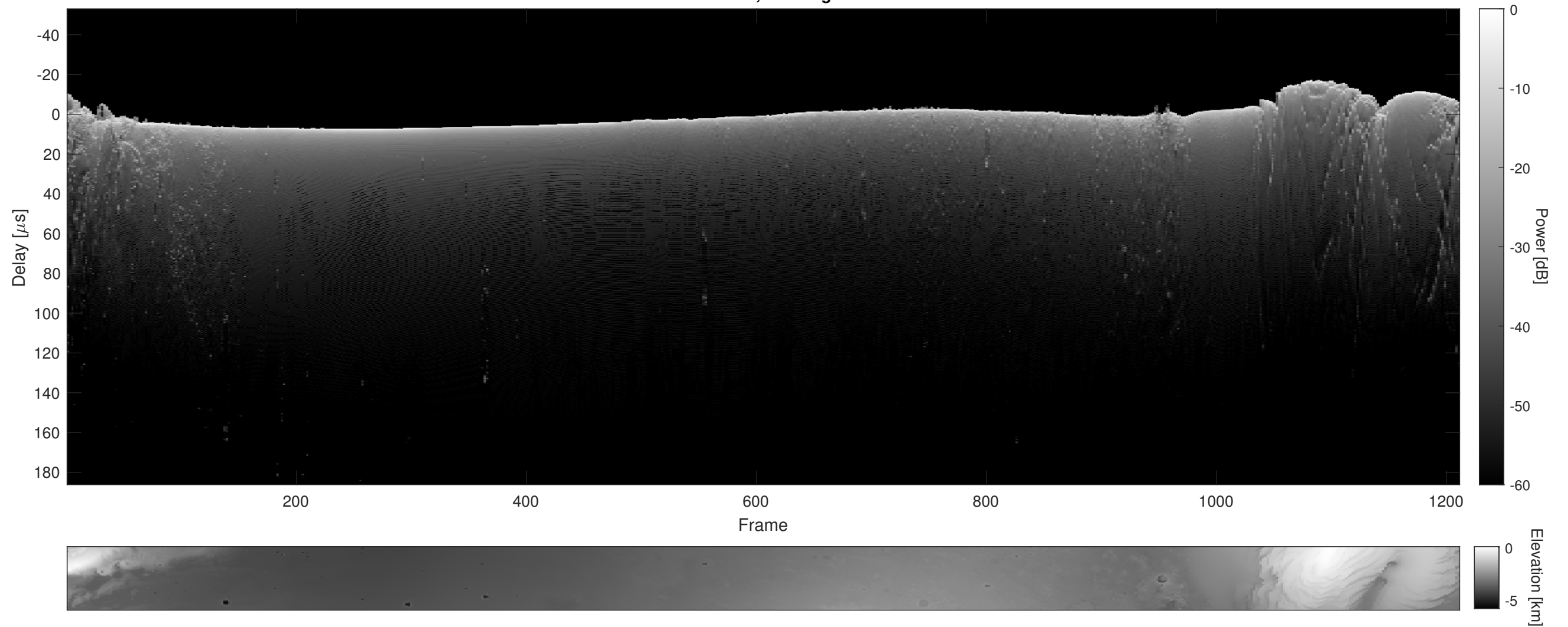
Orbit 10019, Cluttergram
