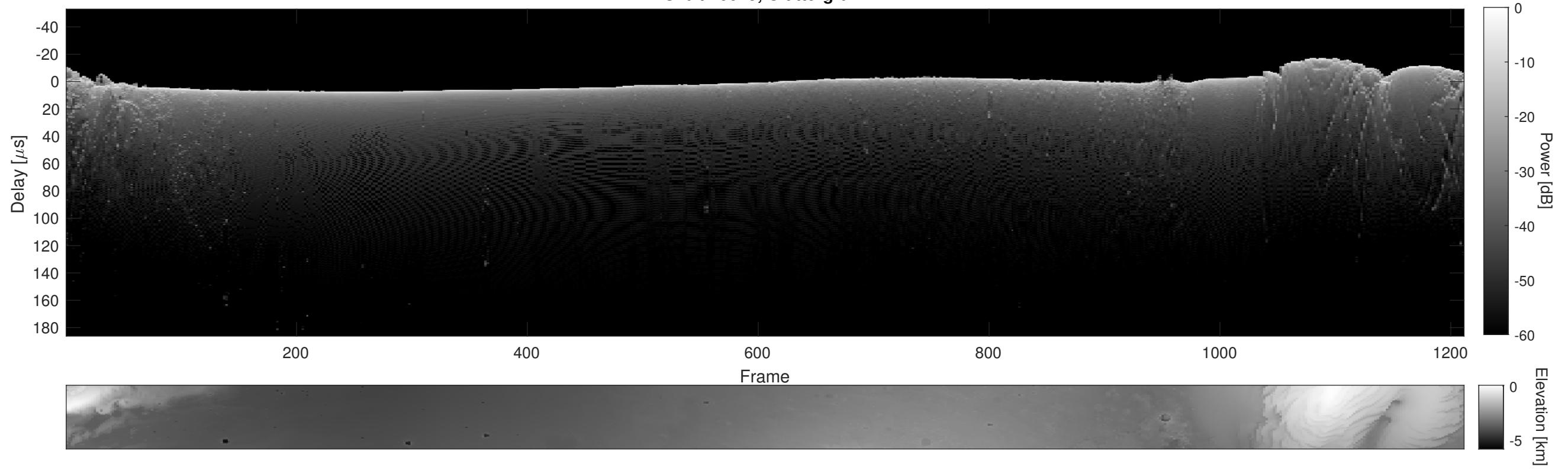
Orbit 10019, Cluttergram
