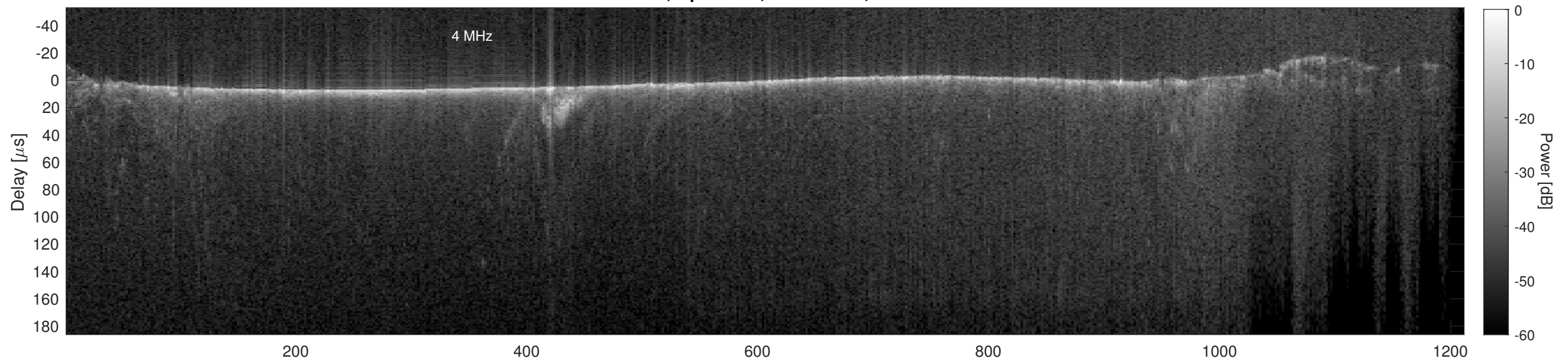
Orbit 10019, Cluttergram
