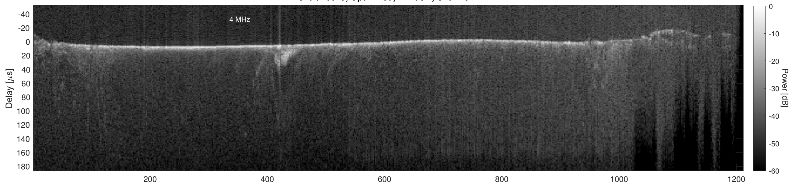
Orbit 10019, Cluttergram
