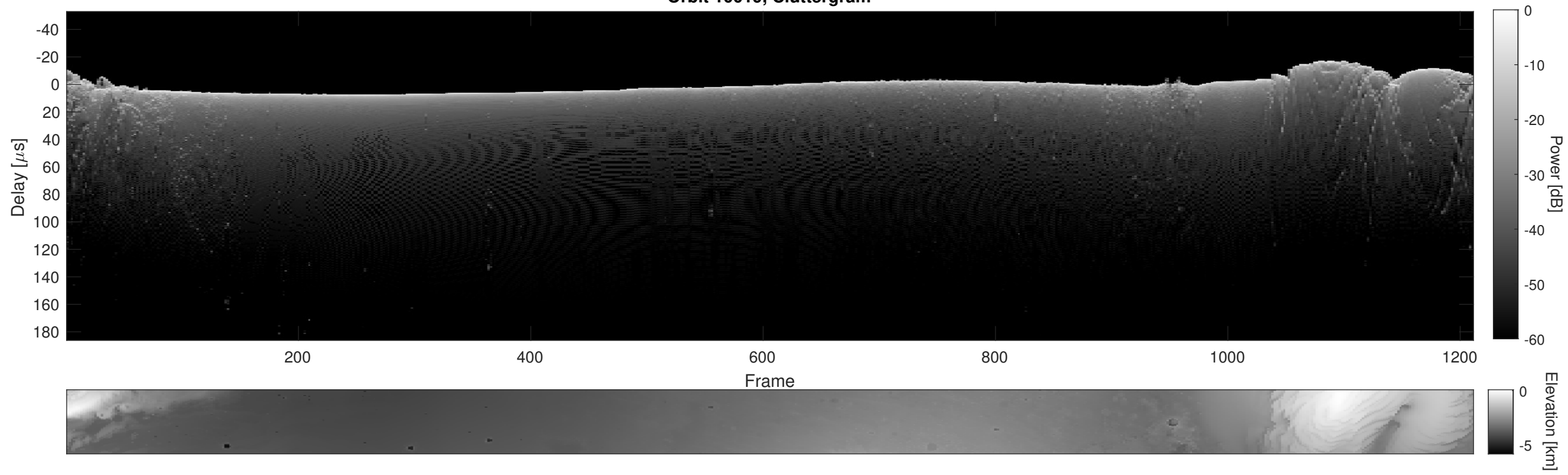
Orbit 10019, Cluttergram
