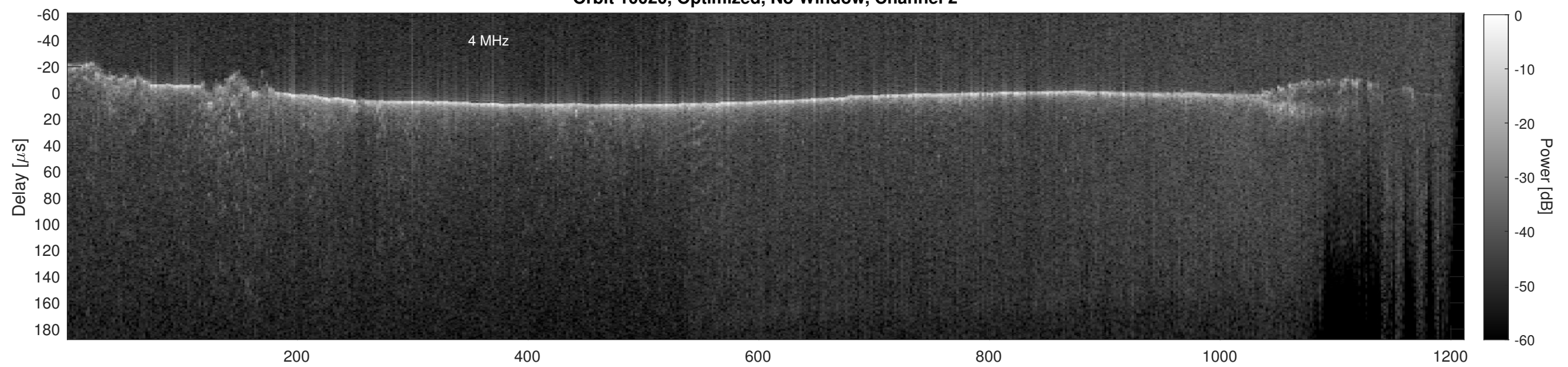
Orbit 10020, Cluttergram
