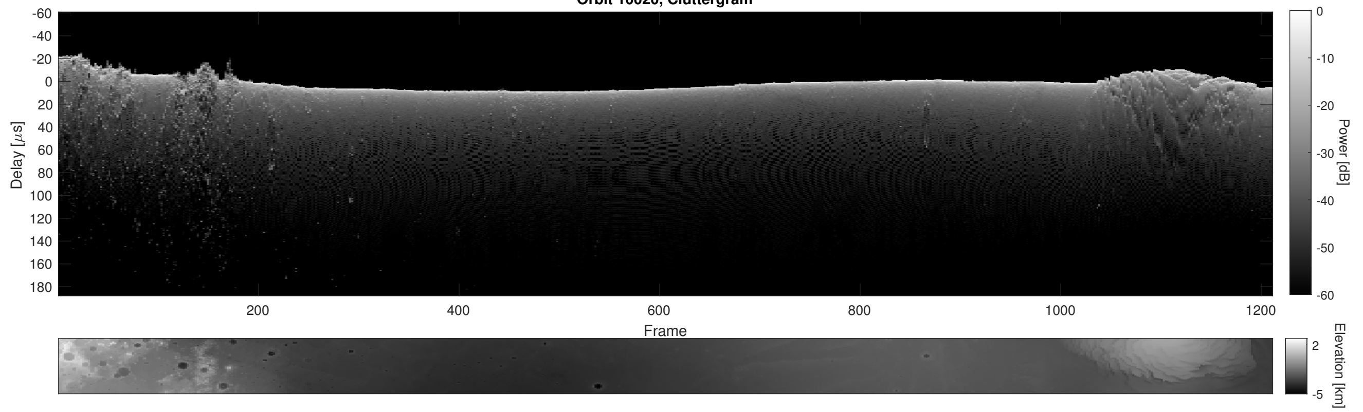
Orbit 10020, Cluttergram
