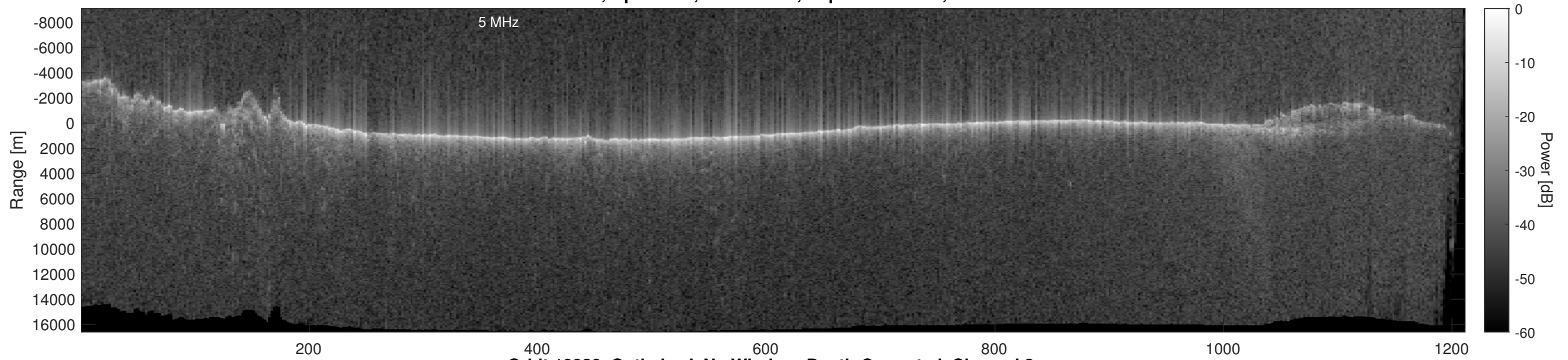
Orbit 10020, Optimized, No Window, Depth-Corrected, Channel 2
