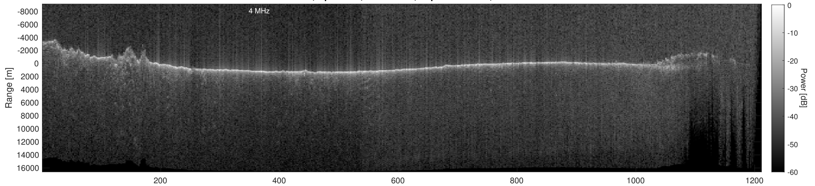
Orbit 10020, Depth-Corrected Cluttergram
