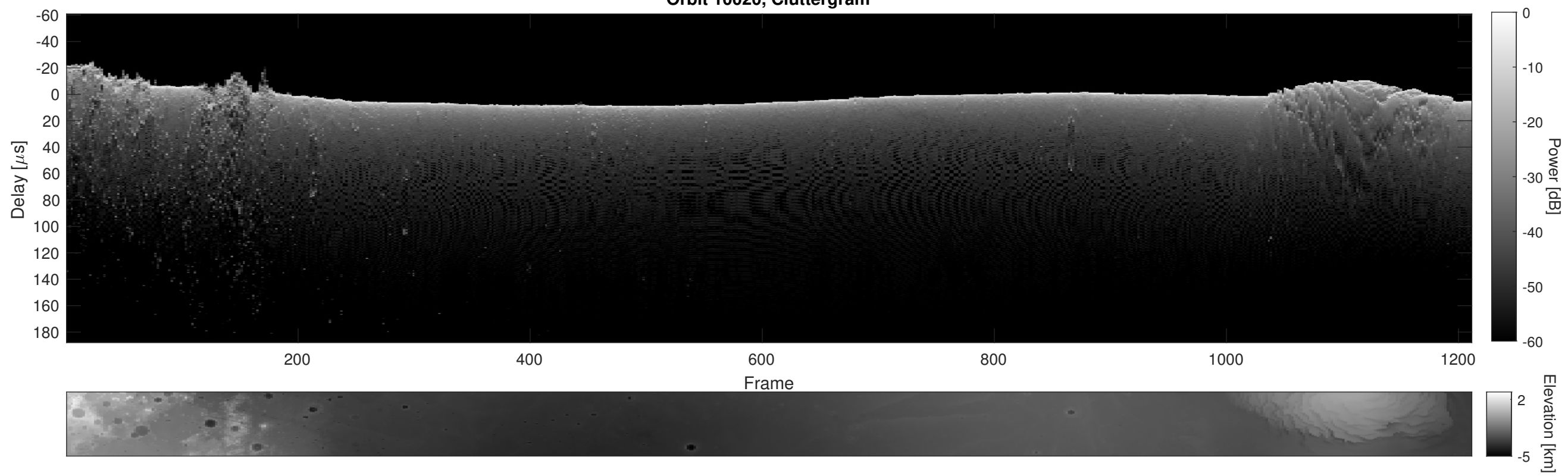
Orbit 10020, Cluttergram
