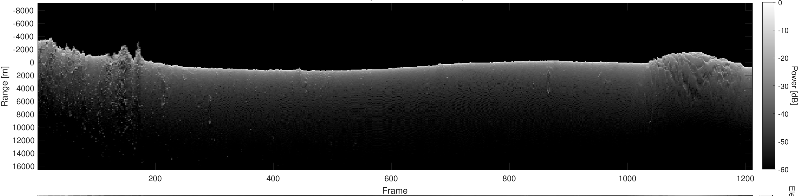
Orbit 10020, Depth-Corrected Cluttergram
