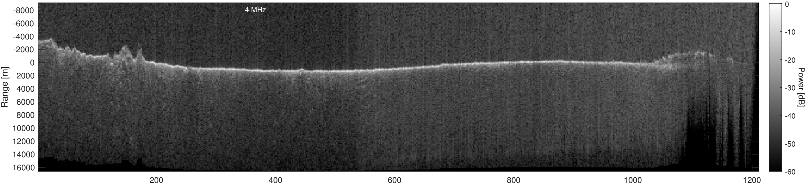
Orbit 10020, Depth-Corrected Cluttergram
