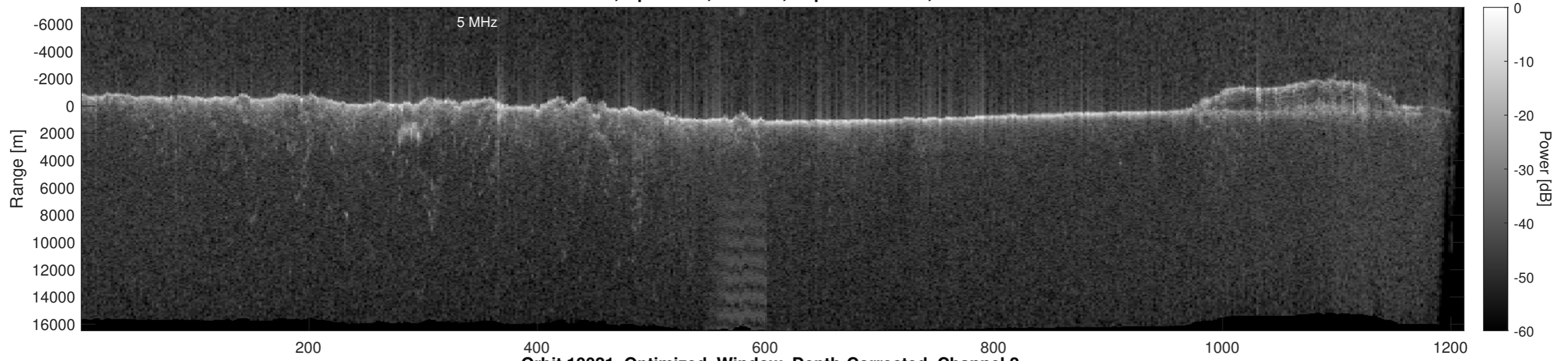
Orbit 10021, Optimized, Window, Depth-Corrected, Channel 2
