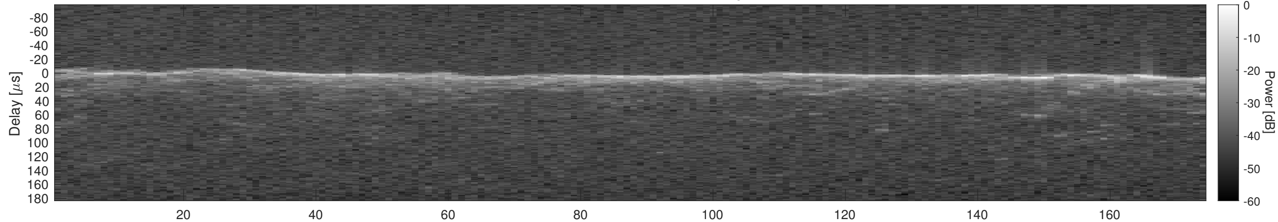
Orbit 10024, Window, Channel 1, Optimized
