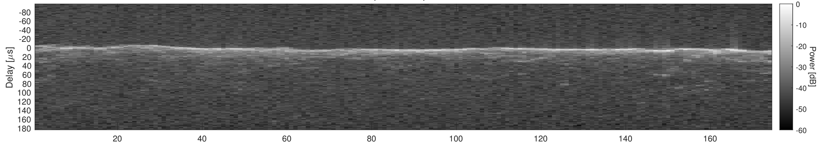
Orbit 10024, Window, Channel 1, Chapman
