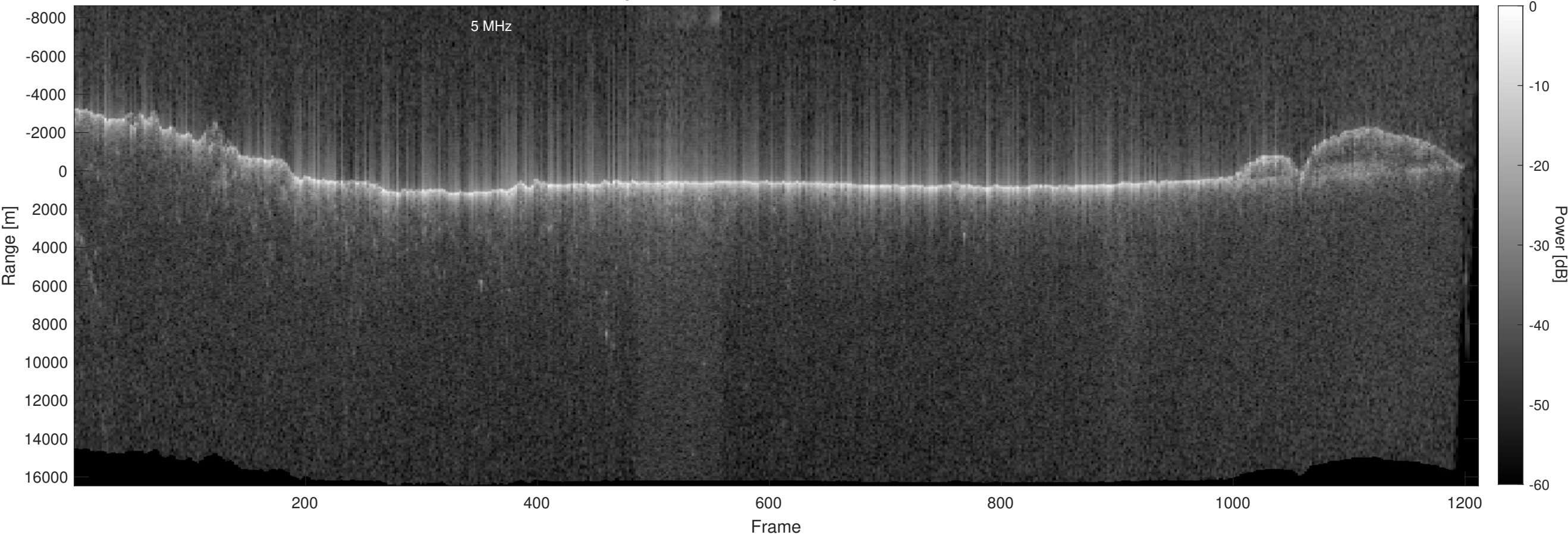
Orbit 10025, Optimized, No Window, Depth-Corrected, Channel 2
