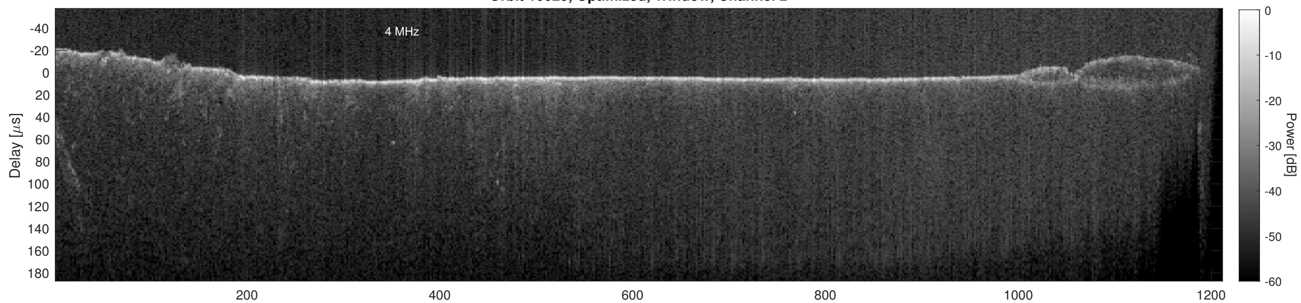
Orbit 10025, Cluttergram
