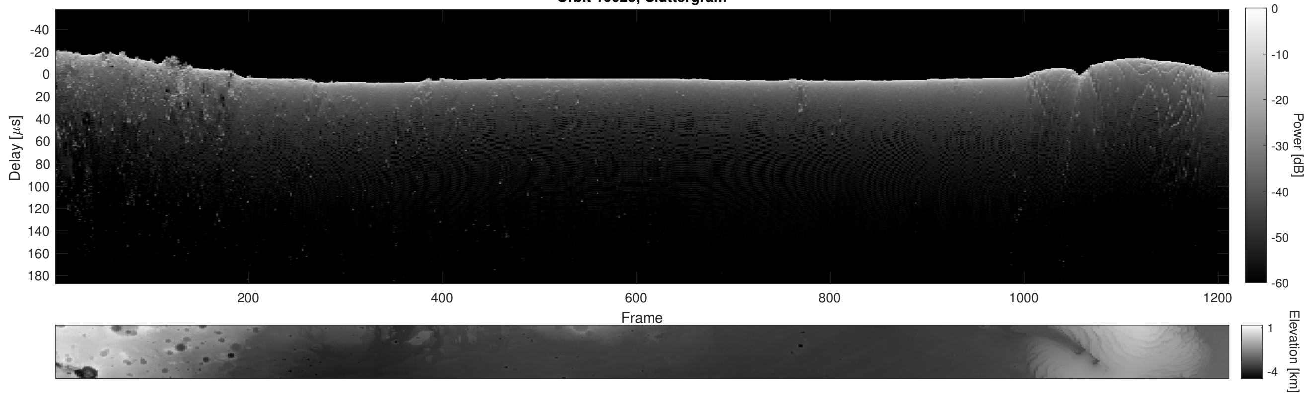
Orbit 10025, Cluttergram
