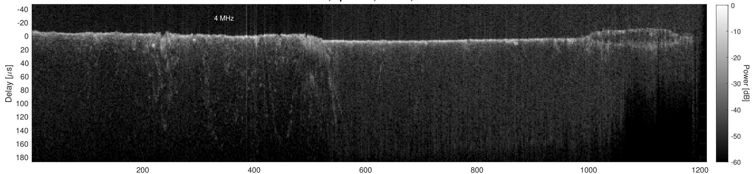
Orbit 10028, Cluttergram
