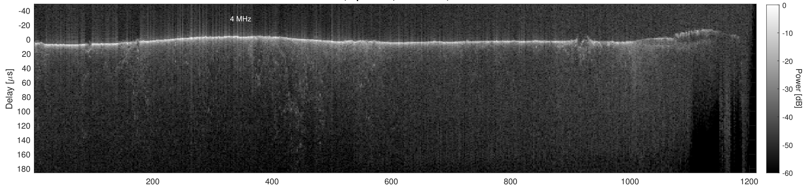
Orbit 10030, Cluttergram
