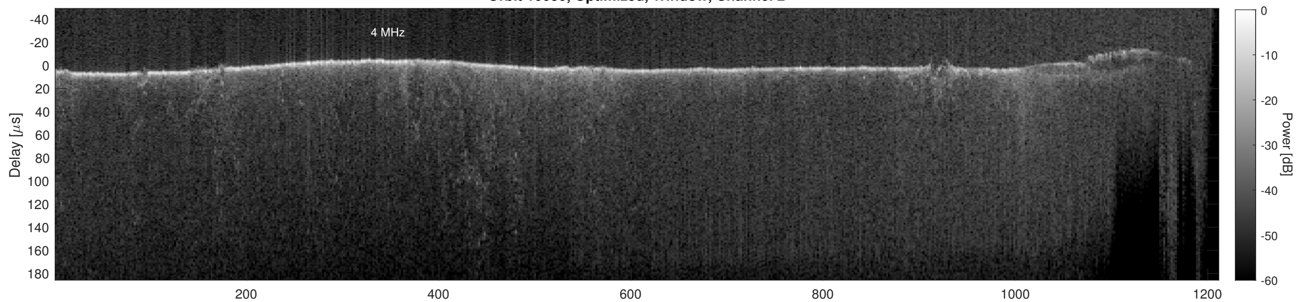
Orbit 10030, Cluttergram
