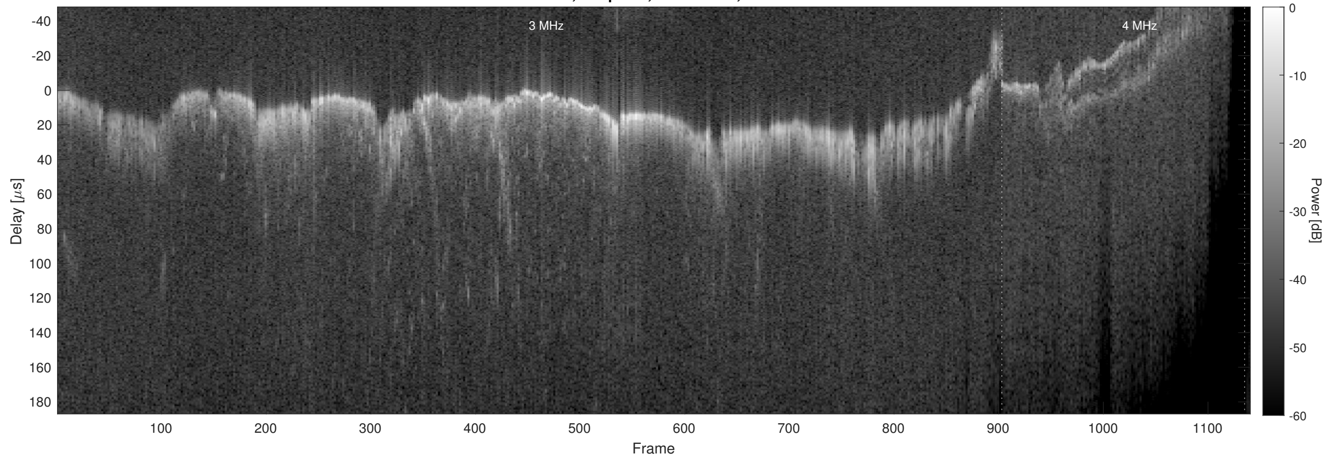
Orbit 10035, Chapman, No Window, Channel 2
