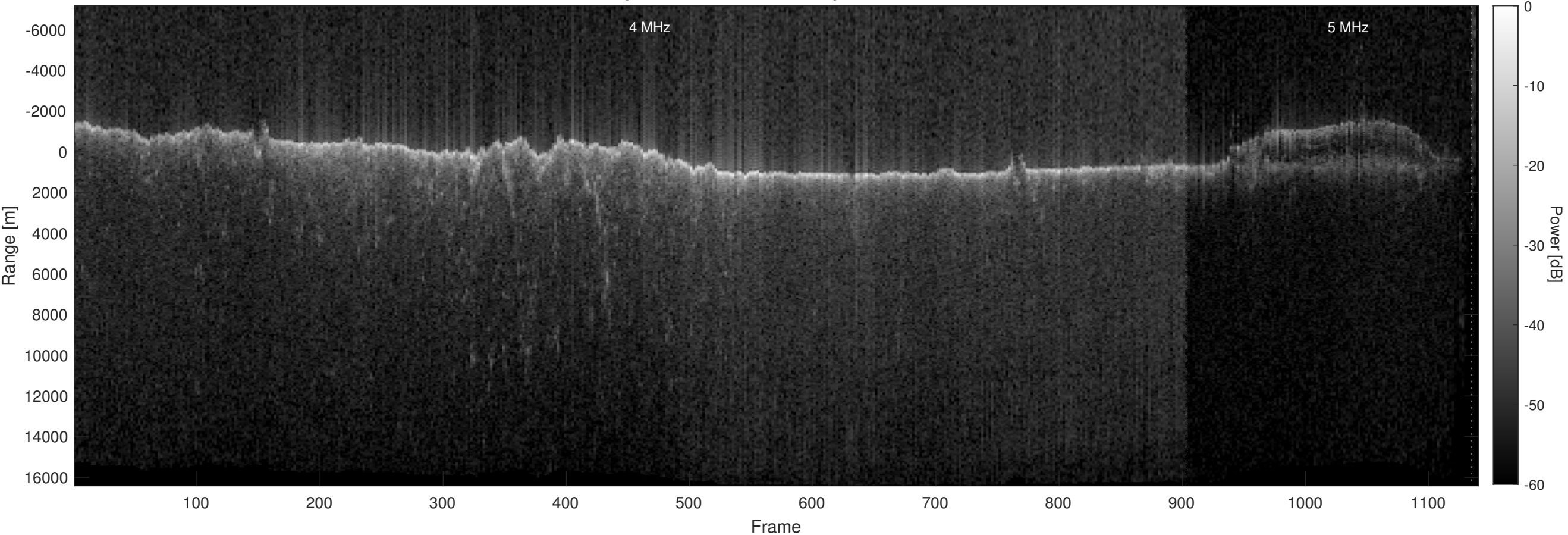
Orbit 10035, Optimized, No Window, Depth-Corrected, Channel 2
