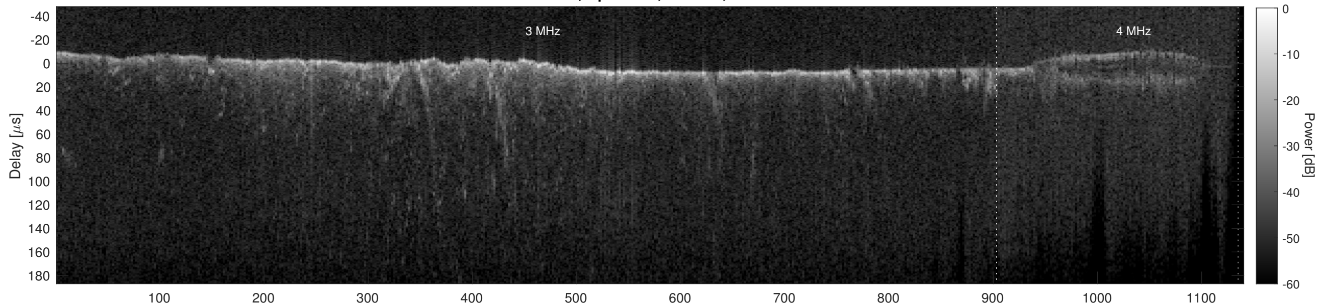
Orbit 10035, Cluttergram
