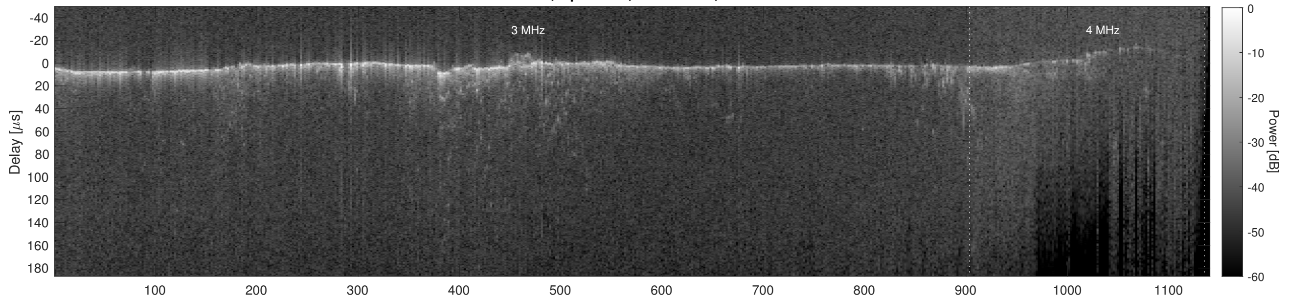
Orbit 10037, Cluttergram
