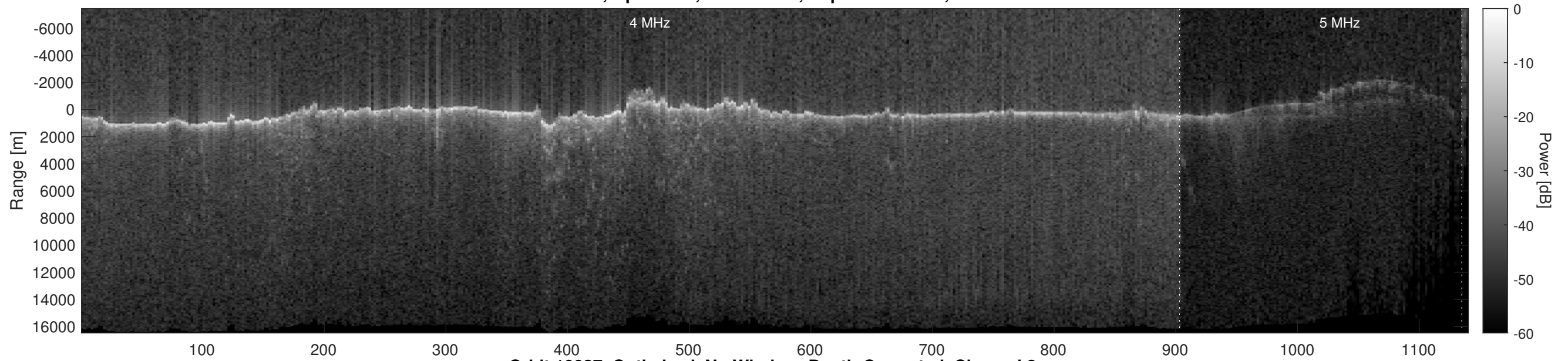
Orbit 10037, Optimized, No Window, Depth-Corrected, Channel 2
