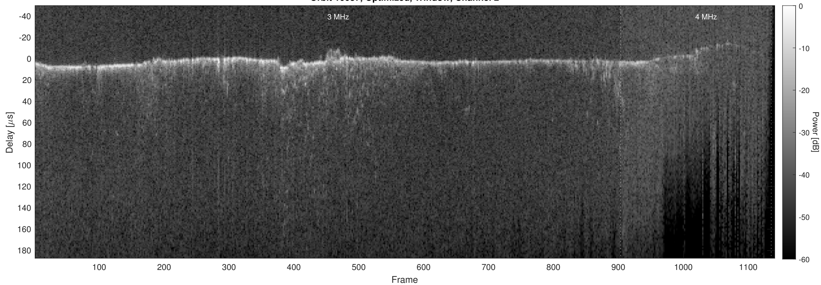
Orbit 10037, Optimized, Window, Channel 2
