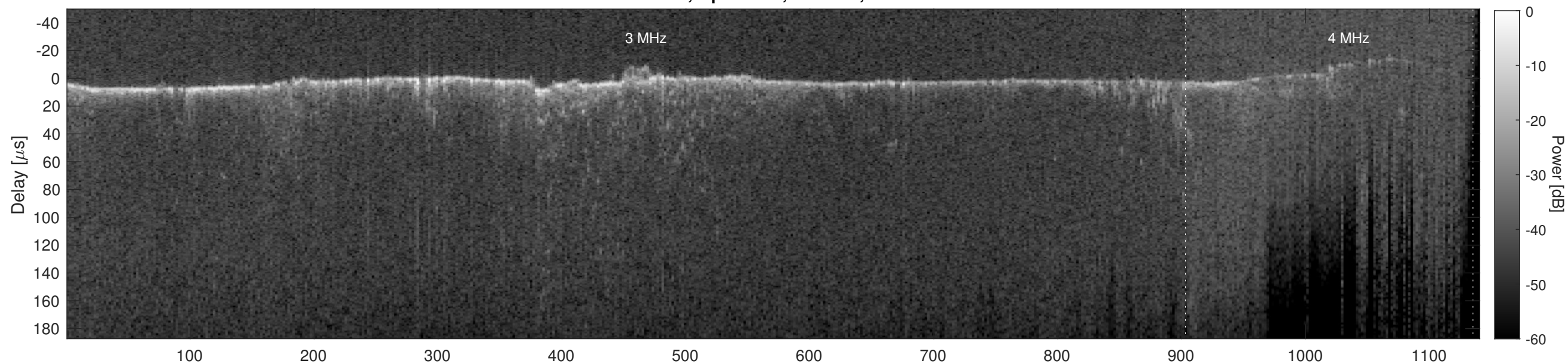
Orbit 10037, Cluttergram
