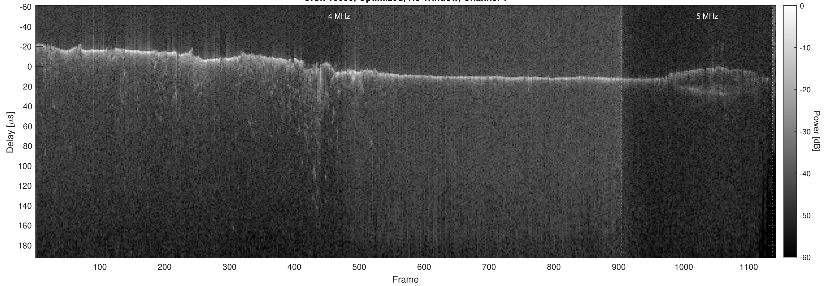
Orbit 10038, Optimized, No Window, Channel 2
