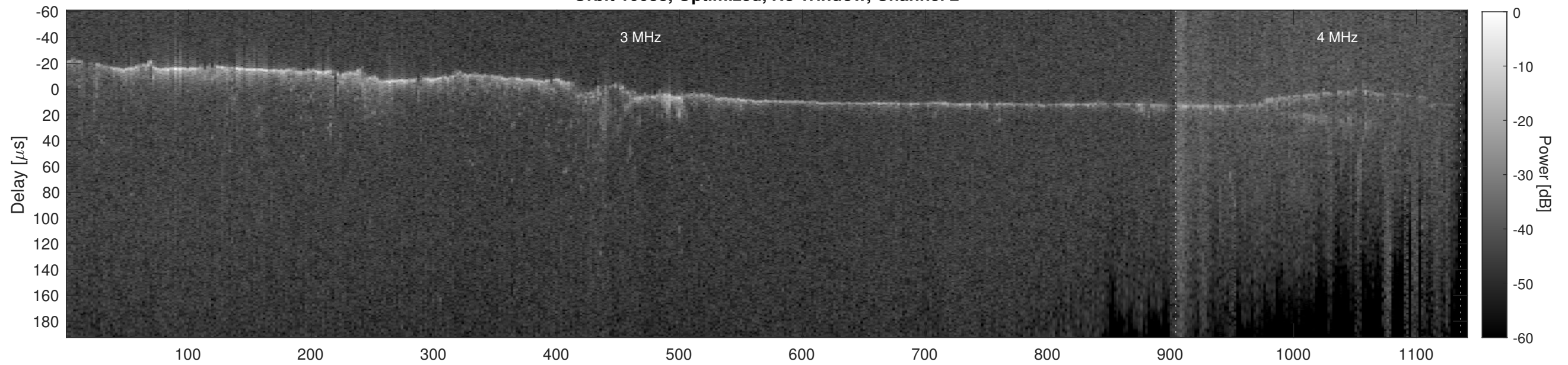
Orbit 10038, Cluttergram
