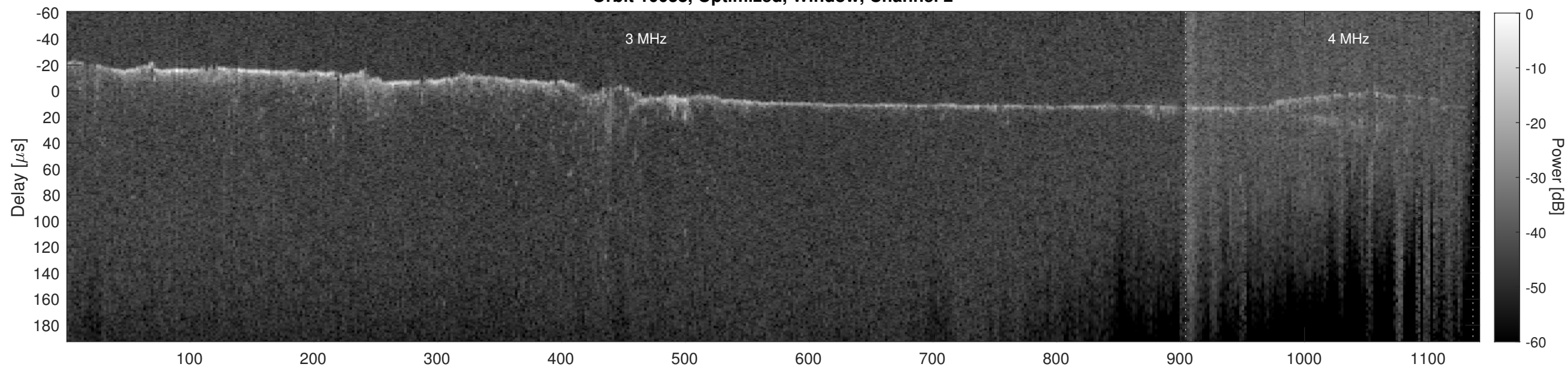
Orbit 10038, Cluttergram
