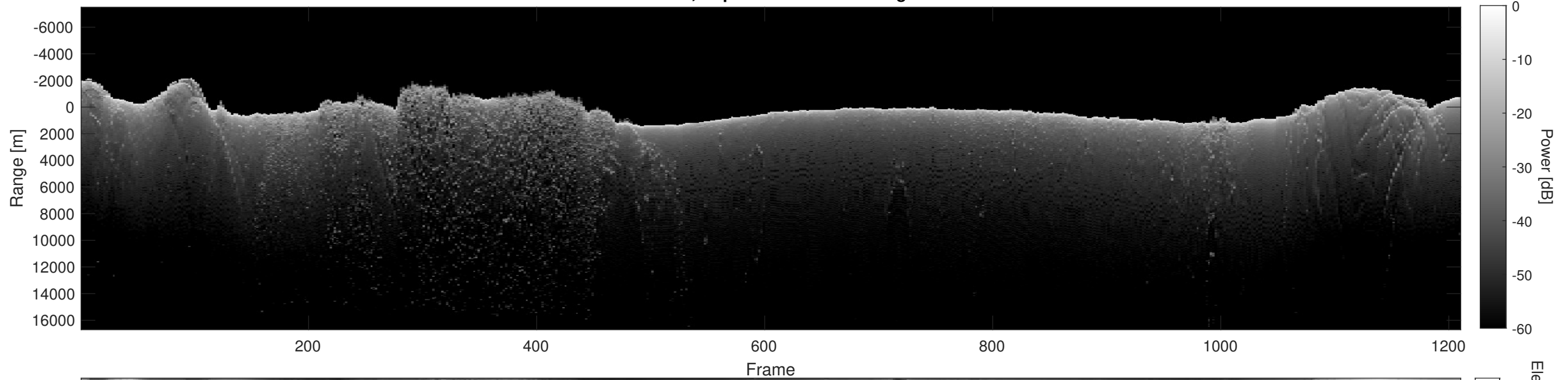
Orbit 10040, Depth-Corrected Cluttergram
