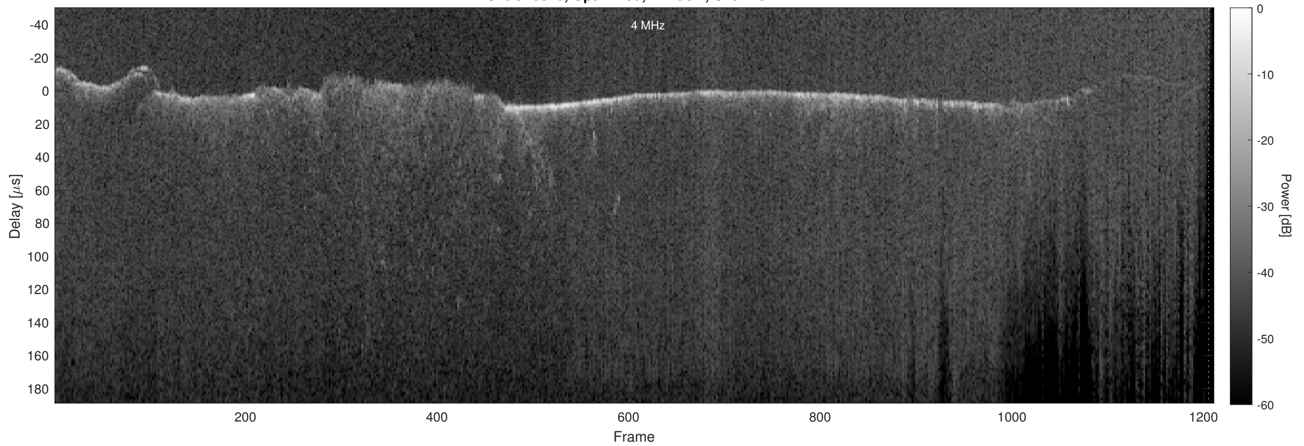
Orbit 10040, Optimized, Window, Channel 2
