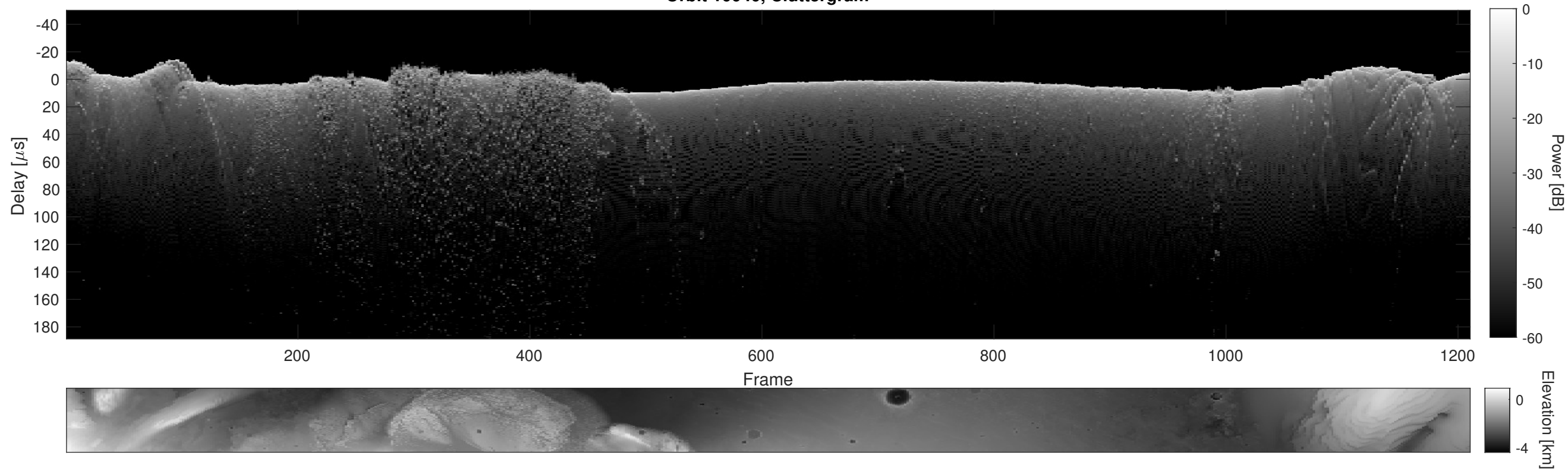
Orbit 10040, Cluttergram
