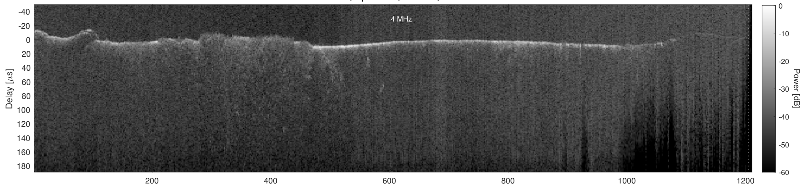
Orbit 10040, Cluttergram
