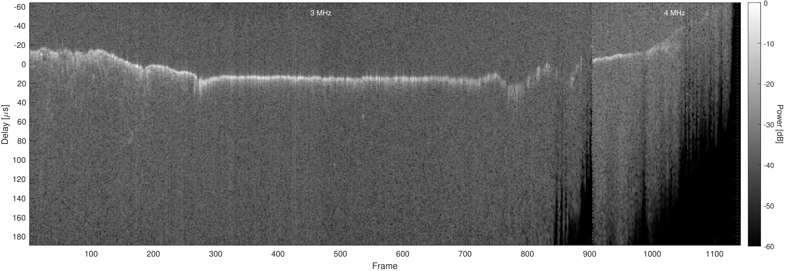
Orbit 10041, Chapman, No Window, Channel 2
