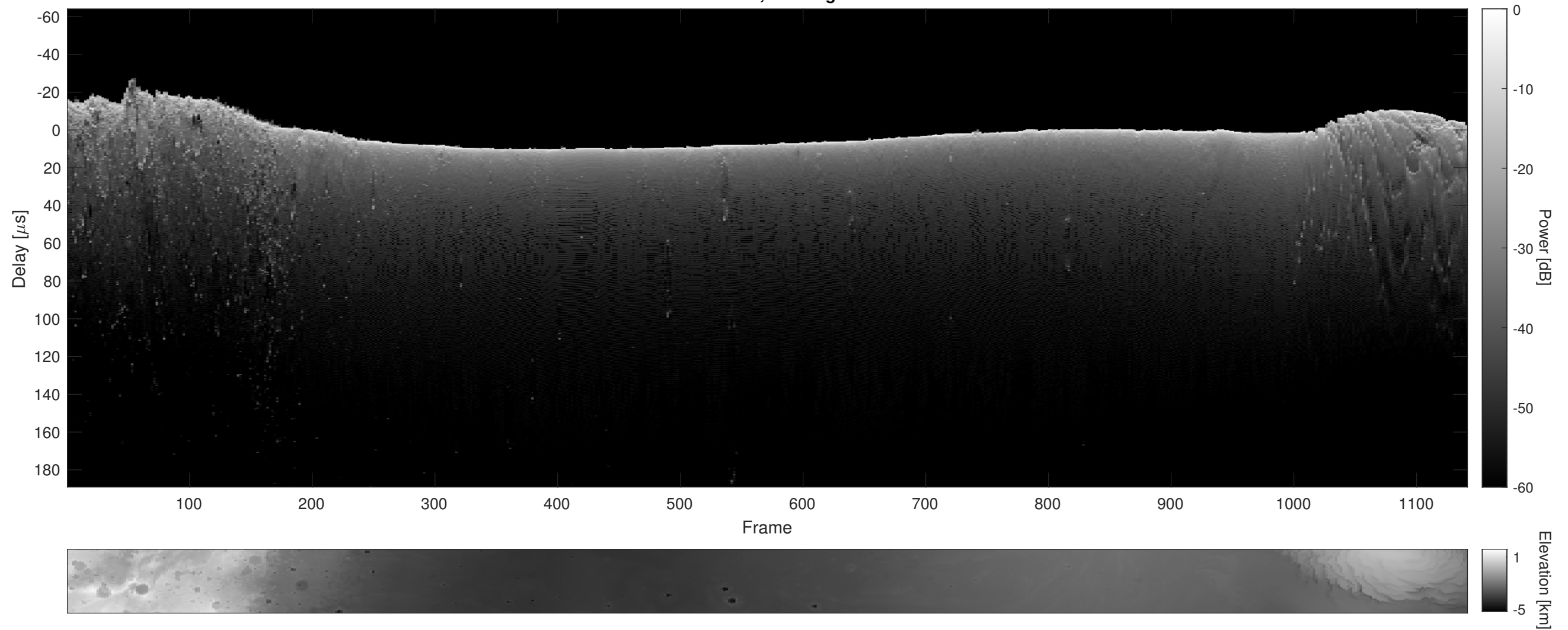
Orbit 10041, Cluttergram
