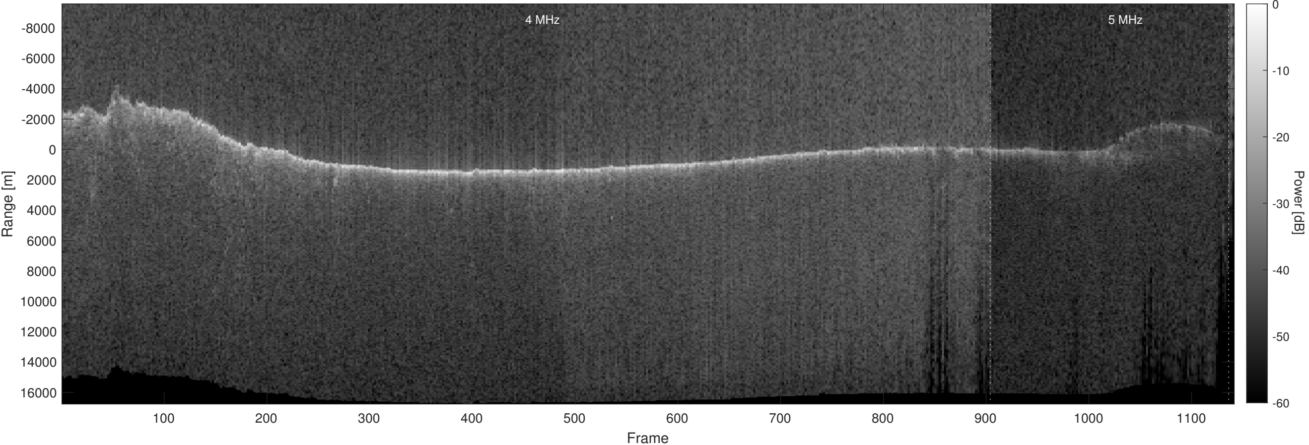
Orbit 10041, Optimized, No Window, Depth-Corrected, Channel 2
