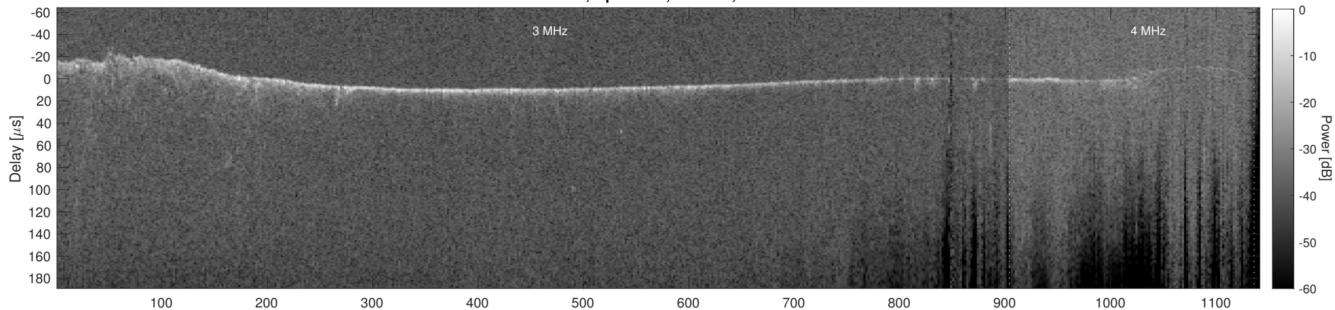
Orbit 10041, Cluttergram
