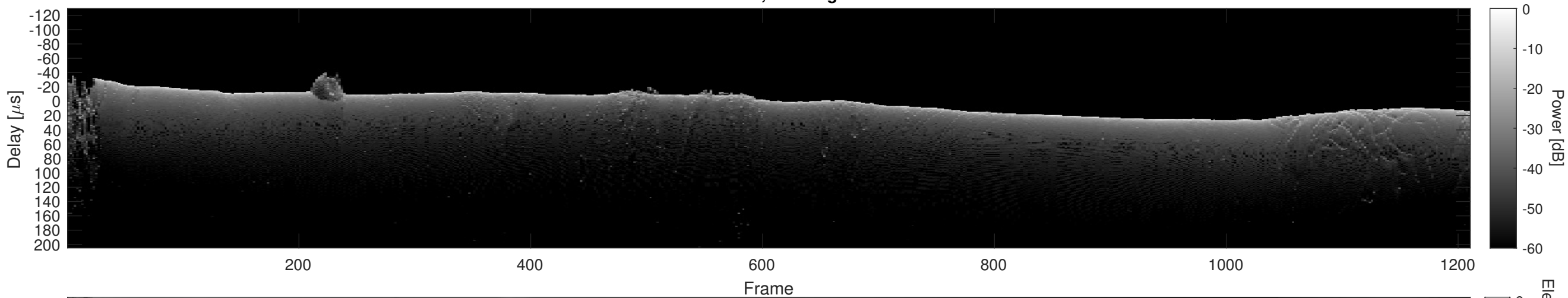
Orbit 10043, Cluttergram
