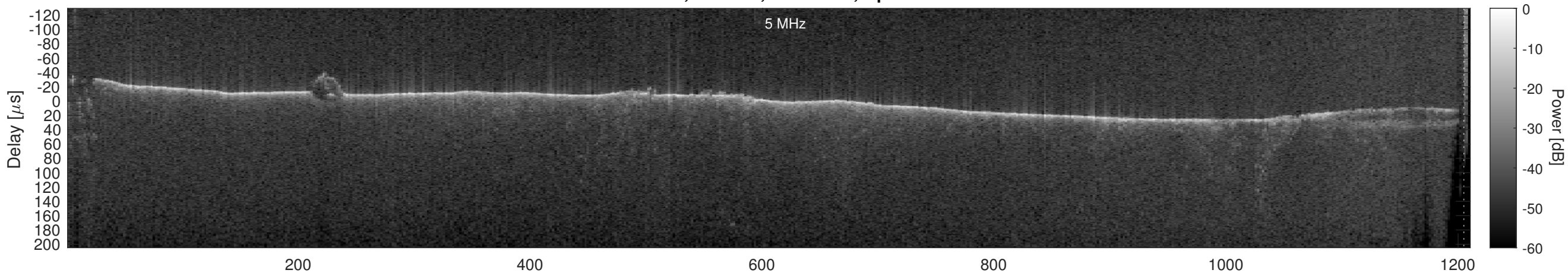
Orbit 10043, Cluttergram
